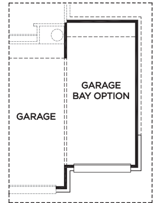
OPTIONAL 3-CAR GARAGE
