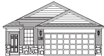
Elevation B (with stone)
